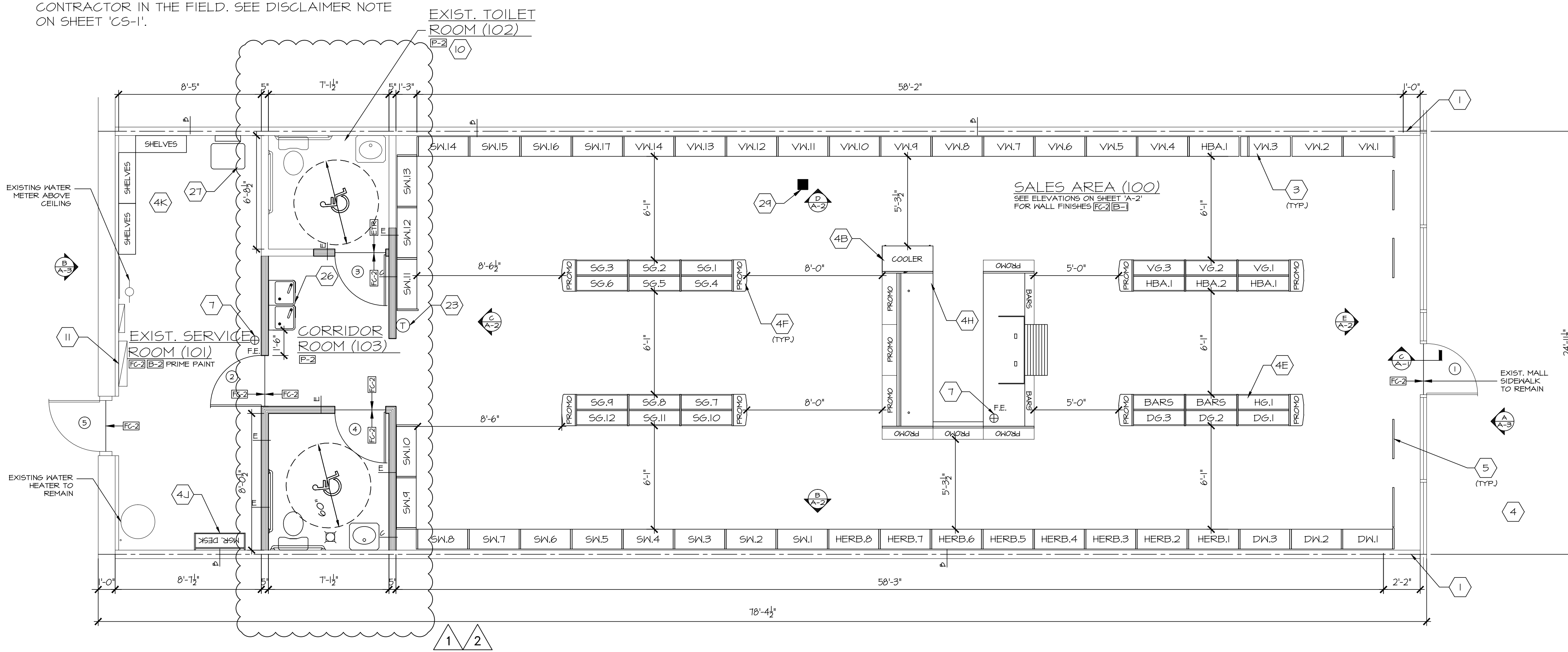
FLOOR PLAN SCALE: 1/4" = 1'-0"
